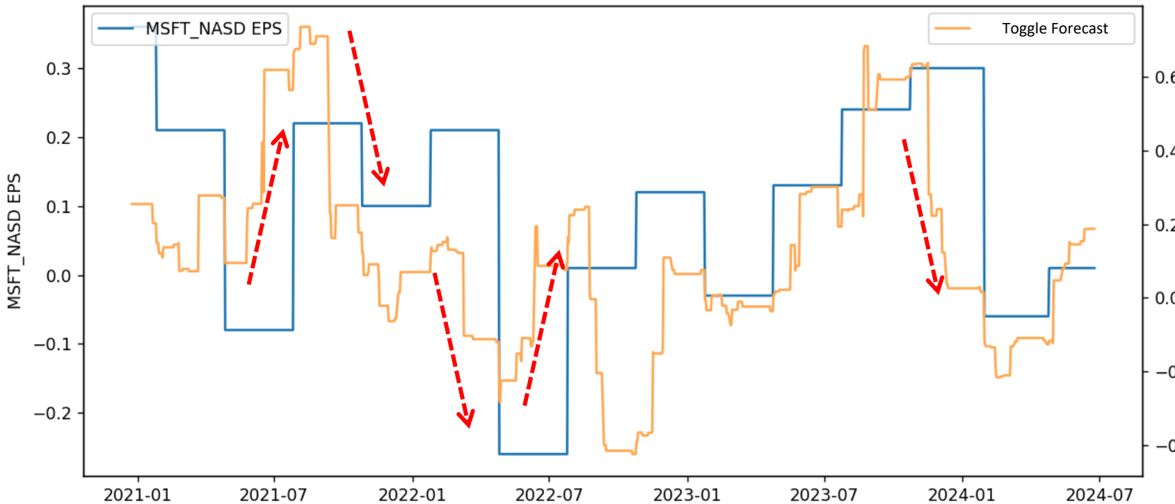
MSFT change in EPS (normalized) vs Toggle Forecast
